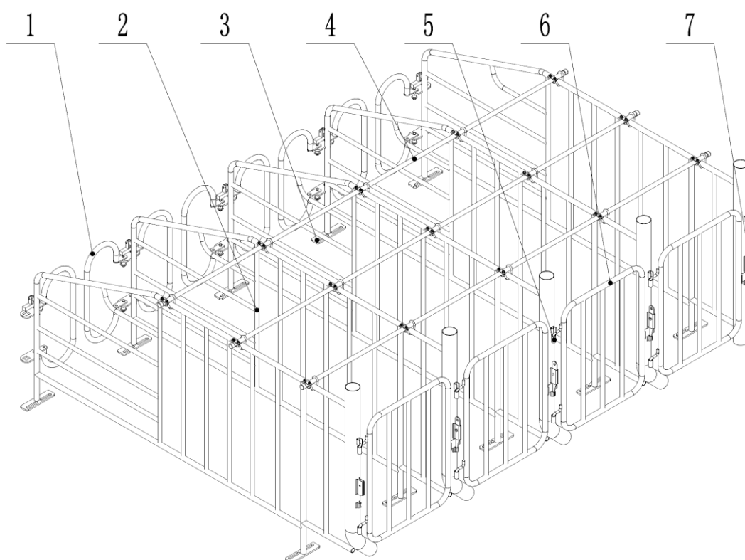
1-后栏门；2-栏片；3-地脚板；4-顶部横杆；5-落料钢管；6-前栏门；7-插销
